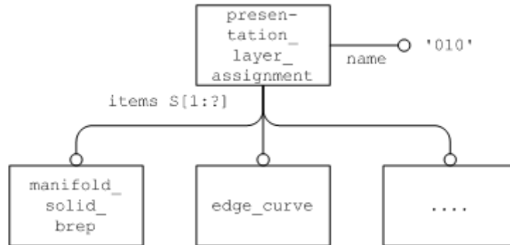
Figure 14: Layer Representation
